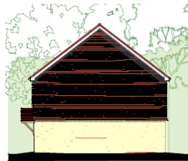
North Elevation Plot 1
